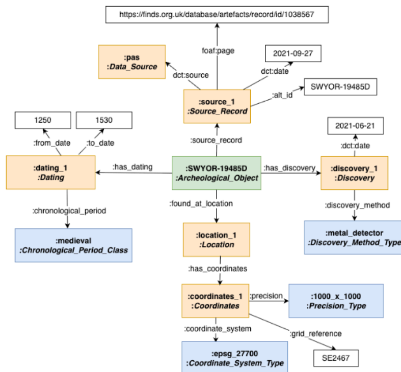
Figure 2: The ARCH-ON data model: intrinsic characteristics
