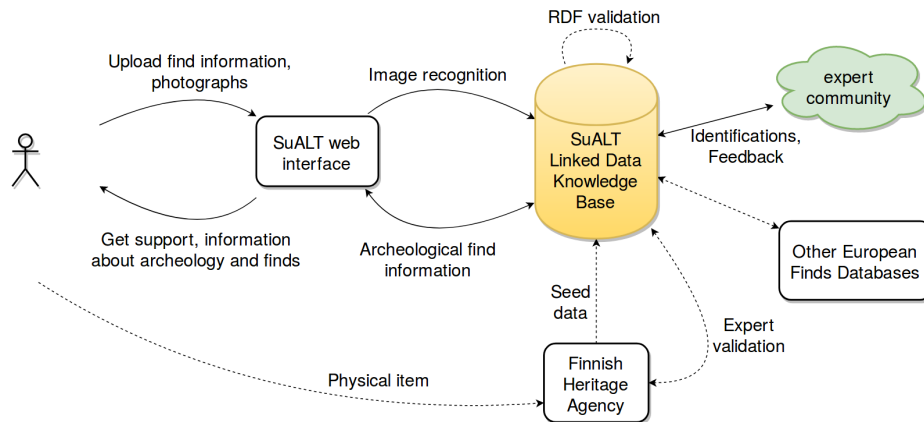
Fig. 1. Workflow in SuALT.
